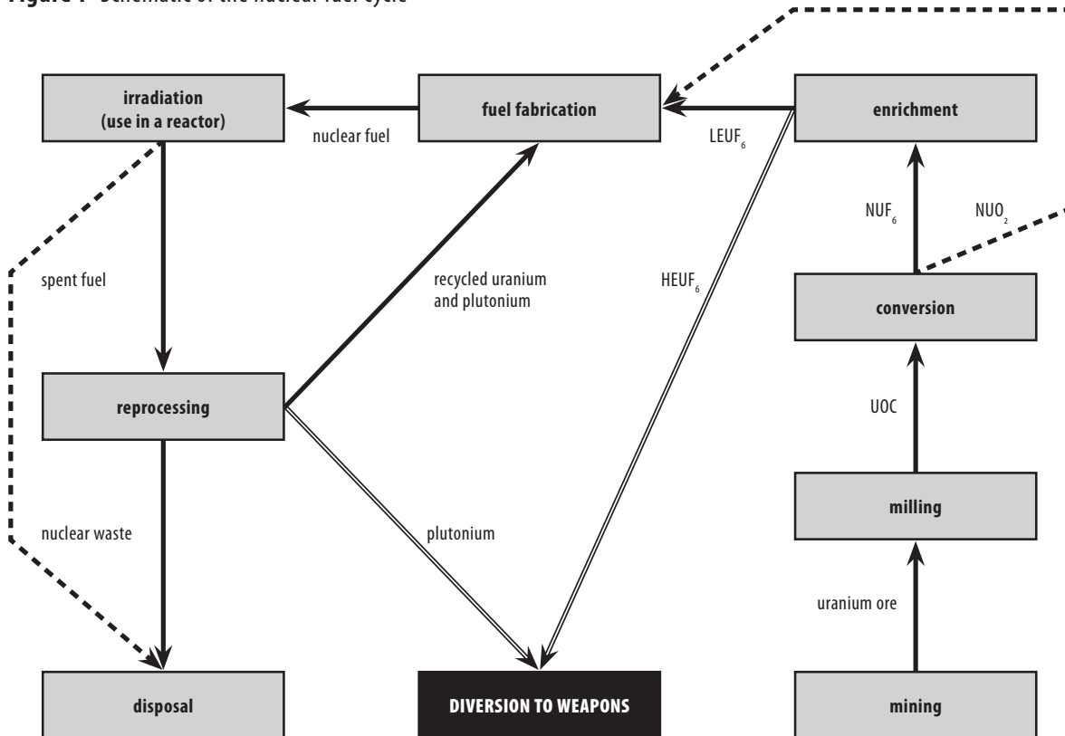
Figure 1 Schematic of the nuclear fuel cycle
