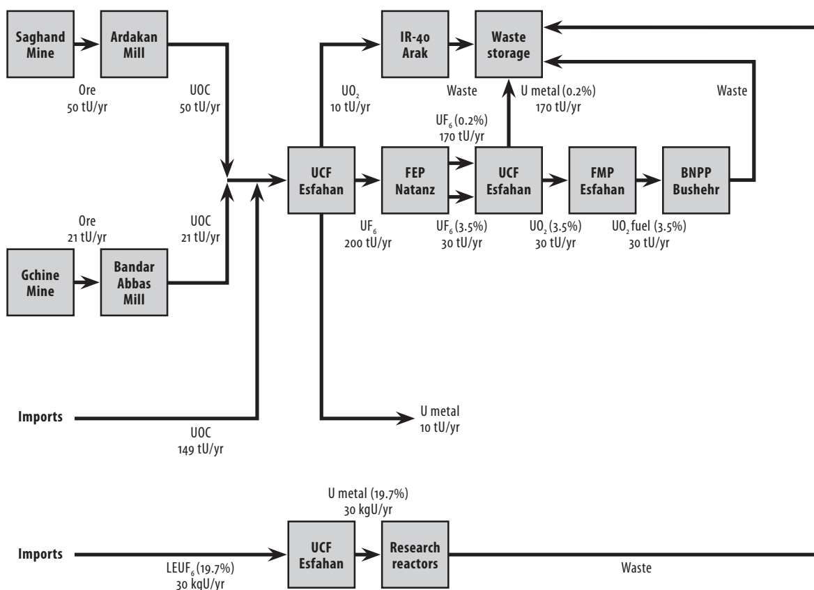
Figure 2 Schematic diagram of Iran's planned fuel cycle activities
